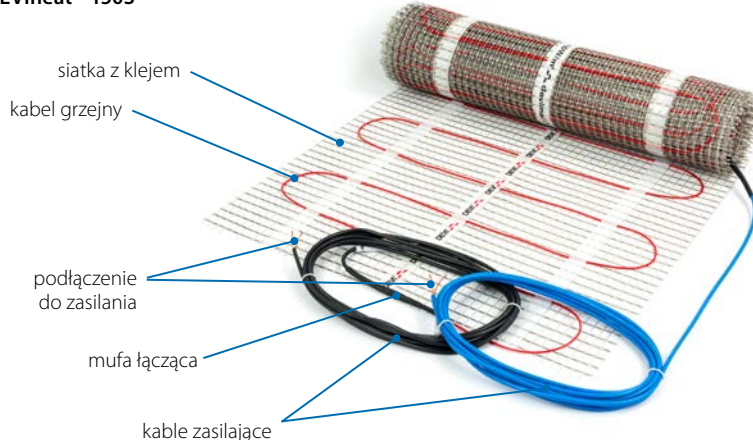
Mata grzejna DEVI ® heat™ 150S
