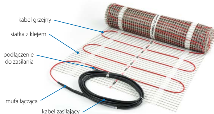
Mata grzejna DEVI ® mat™ 70/100/150/200T
